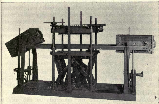
FIG. 10—HAND OPERATED, DOUBLE END, PRESSURE BLOCK MACHINE
